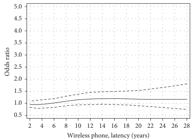
FIGURE 3: Restricted cubic spline plot of the relationship between latency of wireless phones and meningioma. The solid line indicates the OR estimate and the broken lines represent the 95% CI. Adjustment was made for age at diagnosis, gender, socioeconomic index (SEI), and year for diagnosis.
